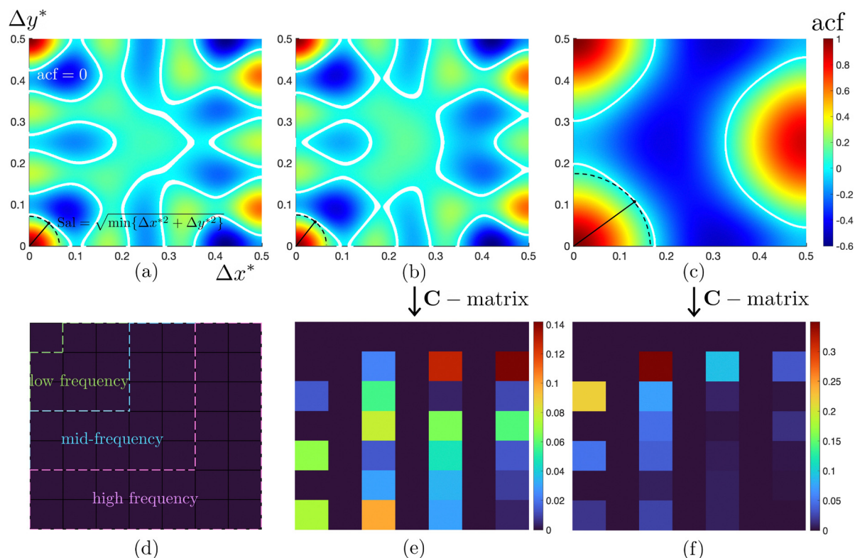
Fig. 9 Normalized autocorrelation function of (a) \min\{(\pi \text{Sq}/\varepsilon_2)^2\} point, r_1 = -2.92 and r_2 = +2.08 . Sal = 0.0692 when (\Delta x^*, \Delta y^*) = (0.042, 0.055) ; (b) \min\{Rku\} point, r_1 = -2.86 and r_2 = +1.98 . Sal = 0.0703 when (\Delta x^*, \Delta y^*) = (0.045, 0.054) ; (c) \min\{\overline{C^{*2}}\} point, r_1 = -1.43 and r_2 = +0.78 . Sal = 0.1691 when (\Delta x^*, \Delta y^*) = (0.131, 0.107) . From (a) to (c), white curves represent acf = 0 . (d) C -Matrix can be split into three zones: low-frequency region, mid-frequency region, and high-frequency region. (e) The contribution heat map of the absolute value of each element in C -matrix for \min\{Rku\} point (corresponding to (b)). The contribution ratio of each region is low : mid : high = 9.4 : 40.3 : 50.3. (f) The same C -matrix visualization for \min\{\overline{C^{*2}}\} point (corresponding to (c)). The contribution ratio of each region is low : mid : high = 64.1 : 24.0 : 11.9. Comparing (e) and (f), we can observe that low frequency dominated profile (64.1%) shows a high Sal , while high frequency dominated profile (50.3%) shows a lower Sal .
