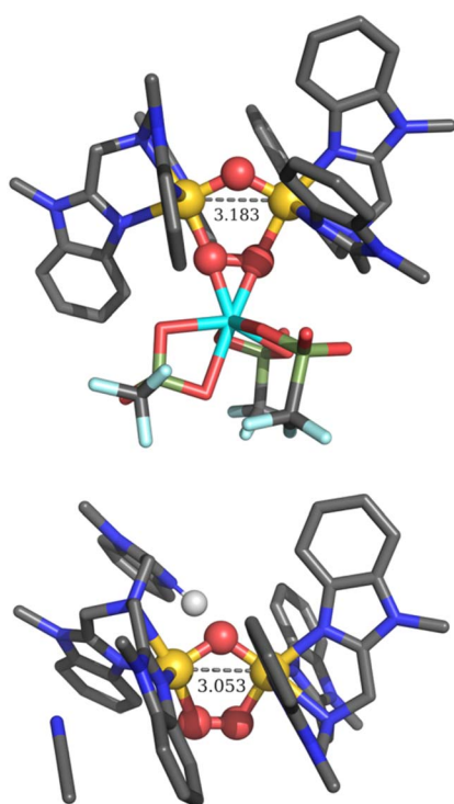
Fig. 3 Top: DFT optimized structure of 2+Sc . Bottom: DFT computed structure (r2scan-3c, COSMO) for 2+H + , which exhibits the short \text{Fe}\cdots\text{Fe} distance as previously inferred from EXAFS analysis. 16
