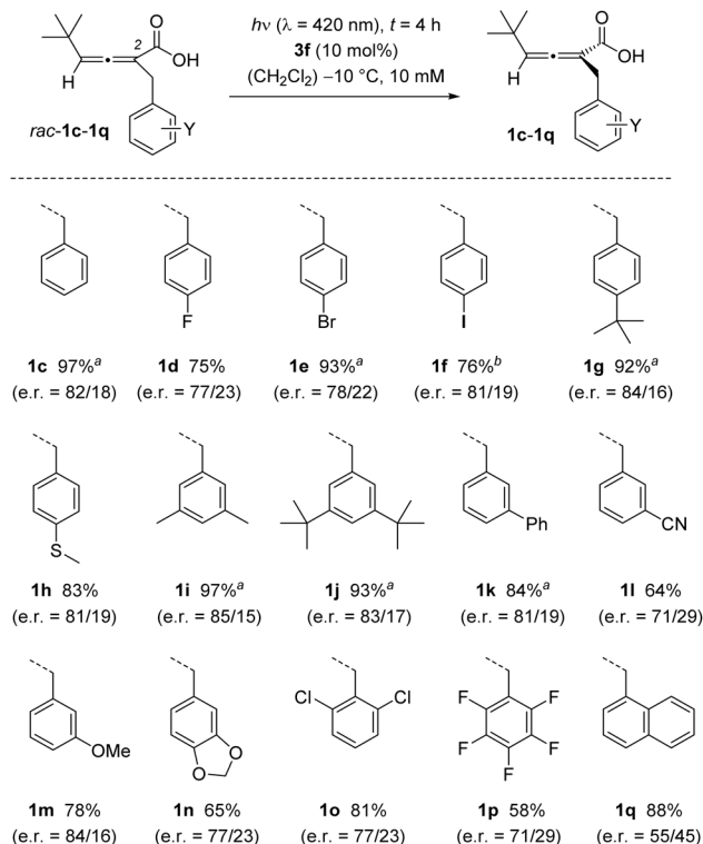
Scheme 3 Photochemical deracemization of 2,3-allenoic acids rac -1c to rac -1q as catalysed by chiral Brønsted acid 3f (50 μmol scale).
