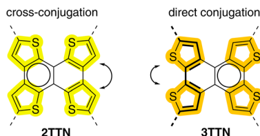
Scheme 1 (a) Thiophene-containing linkers and nodes used in reported COFs. (b) New isomeric naphthotetrathienylene (TTN) nodes reported here.
