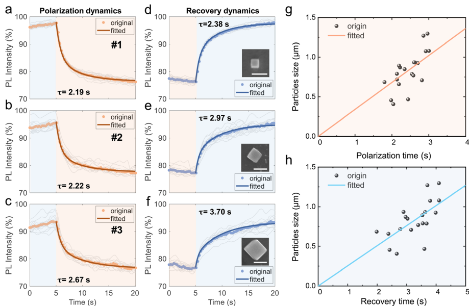
Fig. 2 The polarization and recovery dynamics with different sizes. The polarization process and recovery process of three individuals with side lengths of (a and d) 658 nm, (b and e) 871 nm, and (c and f) 1270 nm at 130 \text{ kV cm}^{-1} . The scale bar is 1 \mu\text{m} . (g and h) Linear correlation of the dynamic time constant with particle size.
