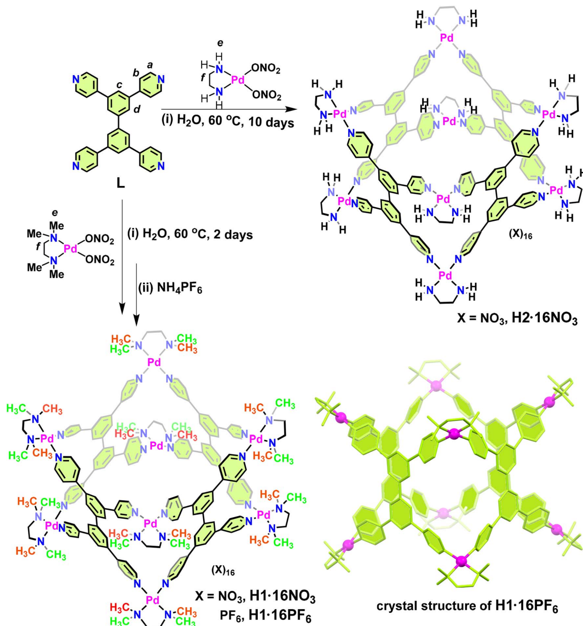
Fig. 2 Synthesis of the polycationic molecular cuboids [\text{Pd}_8(\text{tmeda})_8(\text{L})_4](\text{X})_{16} ( \text{X} = \text{NO}_3 : H1·16NO 3 ; \text{X} = \text{PF}_6 : H1·16PF 6 ), and [\text{Pd}_8(\text{en})_8(\text{L})_4](\text{NO}_3)_{16} , H2·16NO 3 . Crystal structure of H1·16PF 6 showing the [\text{Pd}_8(\text{tmeda})_8(\text{L})_4]^{16+} architecture (counter anions and H atoms are not shown for clarity).
