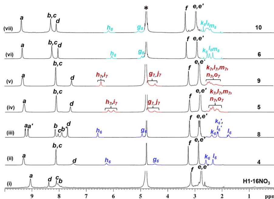
Fig. 6 ^1\text{H} NMR spectra (400 MHz, \text{D}_2\text{O} , 298 K, i.e., 25 ^\circ\text{C} ) for isolated samples of (i) \text{H1}\cdot 16\text{NO}_3 , (ii) [(\text{H6})_2\text{C H1}]\cdot 16\text{NO}_3 (4), (iii) [\text{G}(\text{C}(\text{H6})_2)\text{C H1}]\cdot 17\text{NO}_3 (8), (iv) [(\text{H7})_2\text{C H1}]\cdot 16\text{NO}_3 (5), (v) [\text{G}(\text{C}(\text{H7})_2)\text{C H1}]\cdot 17\text{NO}_3 (9), (vi) [(\text{H8})_2\text{C H1}]\cdot 16\text{NO}_3 (6), and (vii) [\text{G}(\text{C}(\text{H8})_2)\text{C H1}]\cdot 17\text{NO}_3 (10).
