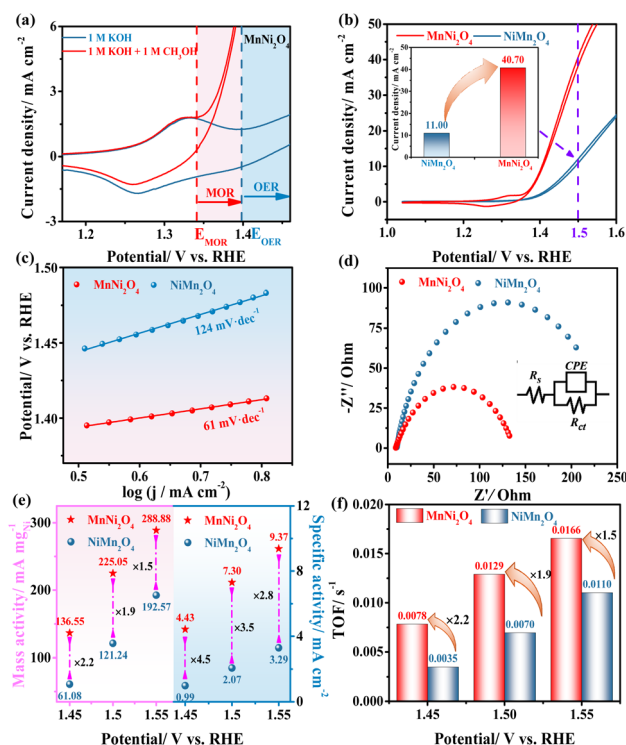
Fig. 3 (a) Cyclic voltammograms of \text{MnNi}_2\text{O}_4 measured in 1 M KOH with and without 1 M \text{CH}_3\text{OH} at 50 \text{mV s}^{-1} . (b) CV curves of \text{NiMn}_2\text{O}_4 and \text{MnNi}_2\text{O}_4 measured in 1 M KOH with 1 M \text{CH}_3\text{OH} at 50 \text{mV s}^{-1} (inset: current density at 1.50 V vs. RHE). (c) Tafel plots of \text{NiMn}_2\text{O}_4 and \text{MnNi}_2\text{O}_4 . (d) Nyquist plots of \text{NiMn}_2\text{O}_4 and \text{MnNi}_2\text{O}_4 at 1.56 V vs. RHE (inset: an equivalent circuit model used for fitting the EIS data). (e) Mass activity and specific activity. (f) TOF of \text{NiMn}_2\text{O}_4 and \text{MnNi}_2\text{O}_4 at 1.45, 1.50, and 1.55 V vs. RHE.
