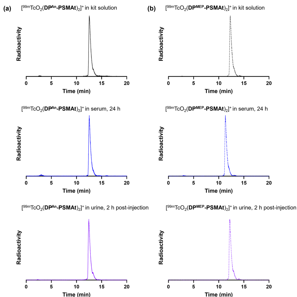
Fig. 3 Radiochromatograms of reactions containing (a) [^{99m}\text{TcO}_2(\text{DP}^{\text{An}}\text{-PSMA})_2]^+ and (b) [^{99m}\text{TcO}_2(\text{DP}^{\text{MEP}}\text{-PSMA})_2]^+ , including radiochromatograms of ^{99m}\text{Tc} samples after either incubation in human serum at 37 ^\circ\text{C} , or after administration to a mouse, followed by collection of urine 2 hours post-administration. Radio-HPLC analyses of serum and urine samples indicate that ^{99m}\text{Tc} radiotracers possess high stability in the presence of serum proteins and in vivo .
