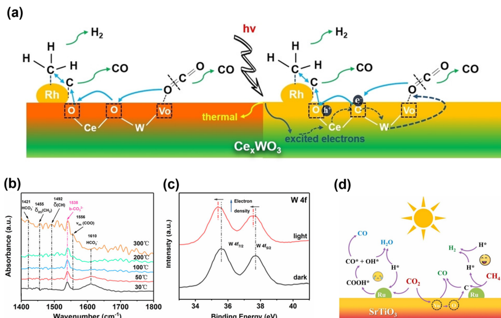
Fig. 12 (a) Schematic diagram for light-driven DRM reaction over Rh/Ce x WO 3 catalyst. (b) In situ DRIFT spectra of Rh/Ce x WO 3 measured in CH 4 /CO 2 mixture under different temperature. (c) XPS spectra of W 4f of Rh/Ce x WO 3 with and without illumination. 116 Copyright 2022, Wiley. (d) Schematic diagram of the photothermal DRM reaction over the Ru/SrTiO 3 catalyst. Adapted with permission from ref. 117 Copyright 2023, Elsevier.
