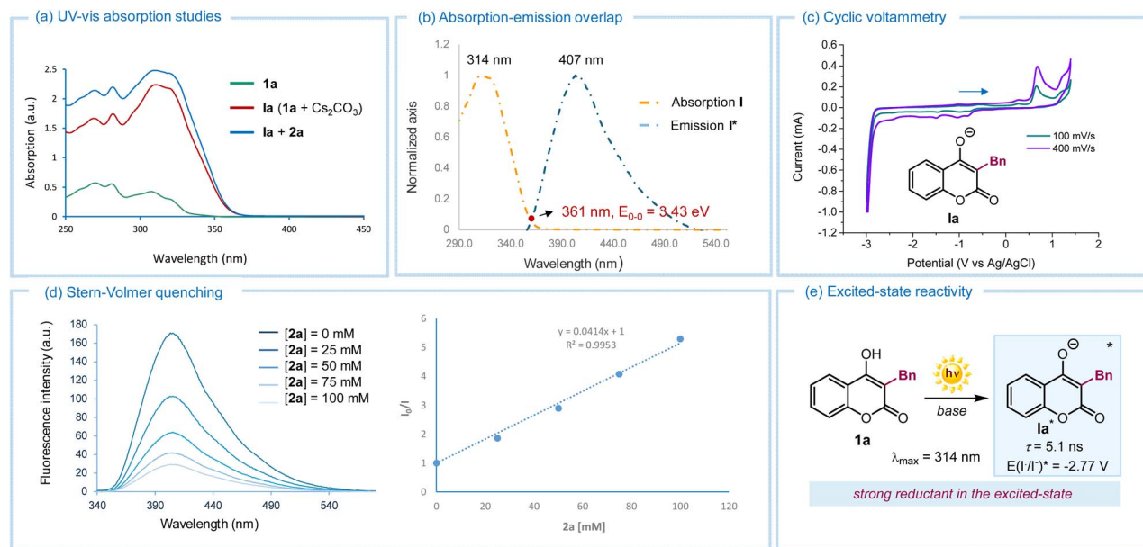
Fig. 2 (a) Absorption spectra recorded for 3-benzyl-4-hydroxycoumarin 1a , its deprotonated form la ( in situ generated from 1a upon addition of Cs 2 CO 3 ), and their mixture with perfluorohexyl iodide 2a in CH 3 CN ( 1 \times 10^{-4} M). (b) Emission of the excited deprotonated intermediate la * in CH 3 CN ( in situ generated mixing 1a with Cs 2 CO 3 ) upon laser irradiation at 314 nm and its intercept at 361 nm with the absorption spectrum, with a 0–0 transition energy ( E_{0,0} ) determined to be 3.43 eV. (c) Cyclic voltammetry measurement of the deprotonated intermediate la carried out in CH 3 CN vs. Ag/AgCl at a scan rate of 100 and 400 mV s −1 . (d) Stern–Volmer luminescence quenching studies of intermediate la ( 1 \times 10^{-4} M in CH 3 CN) with increasing amounts of perfluorohexyl iodide 2a (excitation at 350 nm; emission was acquired from 360 nm to 440 nm).
