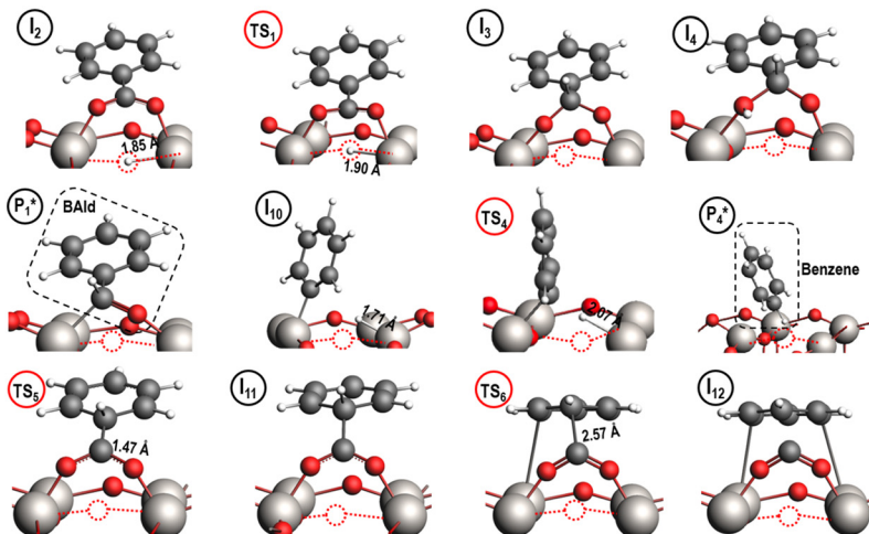
Fig. 5 Reaction energy diagram (a) with optimized intermediate structures (b) of benzoic acid hydrogenation to benzaldehyde and decarboxylation to benzene on reduced anatase TiO 2 (001) with an O vac . Stable intermediate I 1 corresponds to Fig. 3f. All energies are referenced to gas phase benzoic acid and the reduced TiO 2 (001) surface. Structures with gas phase molecules are circled in blue, adsorbed species in black, and transition states in red. Only the uppermost atomic layer is shown for the sake of clarity. Ti (gray), O (red), C (black), H (white), and O vac (dashed circle) are depicted.
