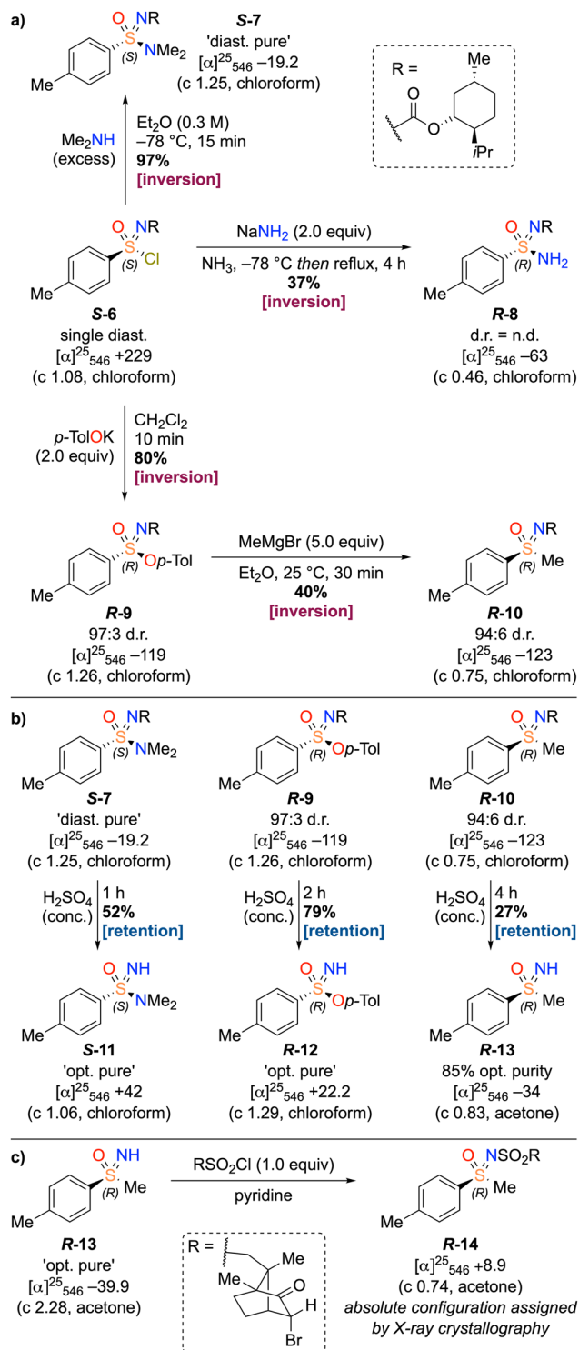
Scheme 2 (a) Synthesis of sulfonamidamides S-7 and R-8 , sulfonimide R-9 and sulfoximine R-10 from diastereomerically pure sulfonimidoyl chloride S-6 ; (b) removal of carbomethoxy chiral auxiliary to afford free NH products; (c) synthesis and configurational assignment of sulfoximine R-14 . n.d. = not determined; 'diast. pure' = compound claimed as diastereomerically pure, no values quoted; 'opt. pure' = compound claimed as optically pure, no values quoted.
