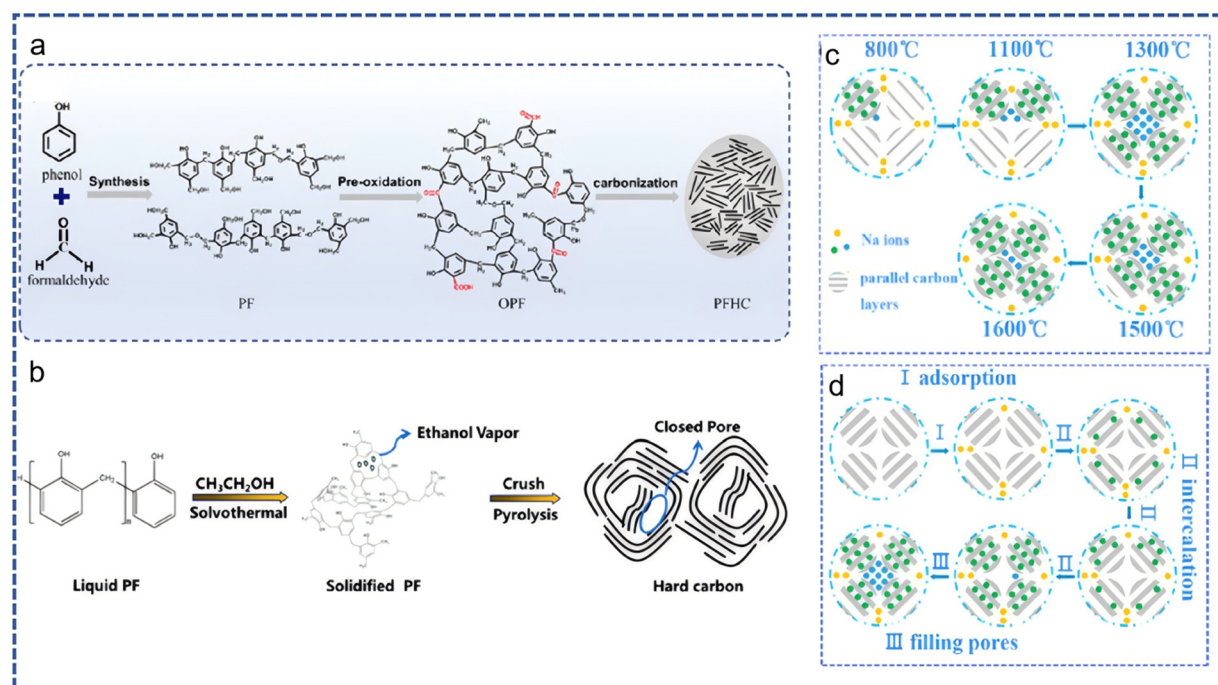
Fig. 19 (a) PF resin synthesis and the HC production process; reproduced with permission from ref. 80; copyright: 2021 American Chemical Society. (b) The HC closed pore formation mechanism; (c) sodium-ion filling as temperature increases; and (d) the sodium-ion filling process; reproduced with permission from ref. 81; copyright: 2024 American Chemical Society.
