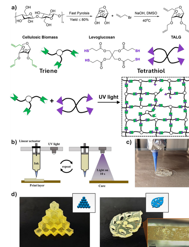
Fig. 14 (a) Schematic diagram of DIW 3D printing ink with triene and tetrathiol as the main components and its photopolymerization reaction. (b) A schematic illustration of the DIW process used for 3D printing. (c) Real-time image capturing the extrusion of TALG-poly3SH-1 resin during printing. (d) Representative 3D printed structures fabricated using the TALG-poly3SH-1 formulation. Reproduced with permission from ref. 181. Copyright 2023, Royal Society of Chemistry.
