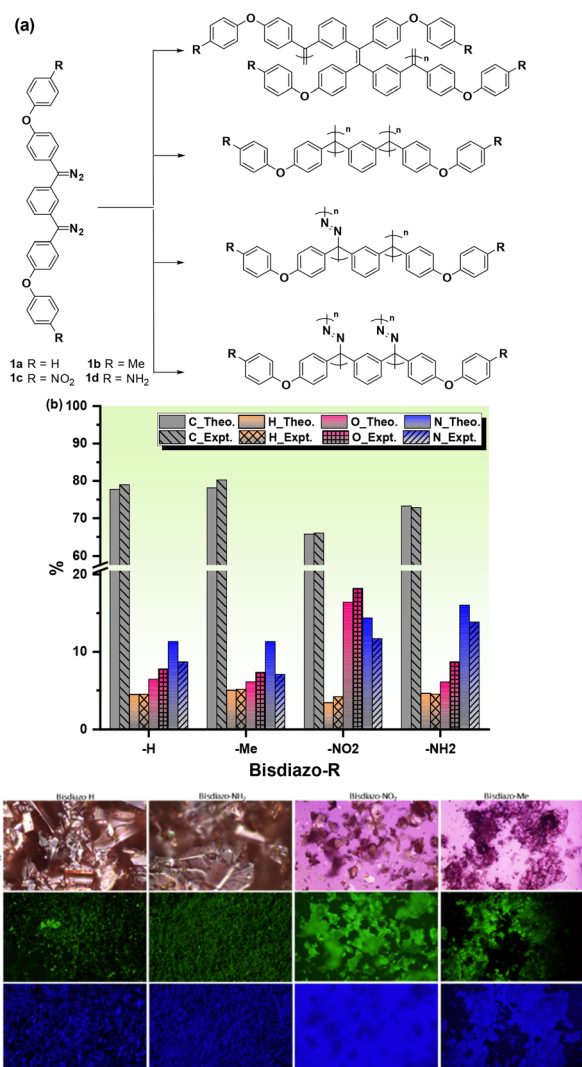
Fig. 1 (a) Chemical structures of bisdiazot-R compounds 1a–d and the possible repeating units of polymers under catalyst-free polymerization. (b) Elemental analysis and (c) optical and fluorescence images of bisdiazot-R compounds 1a–d with various terminal groups ( R = H , Me , NO_2 and NH_2 ).
