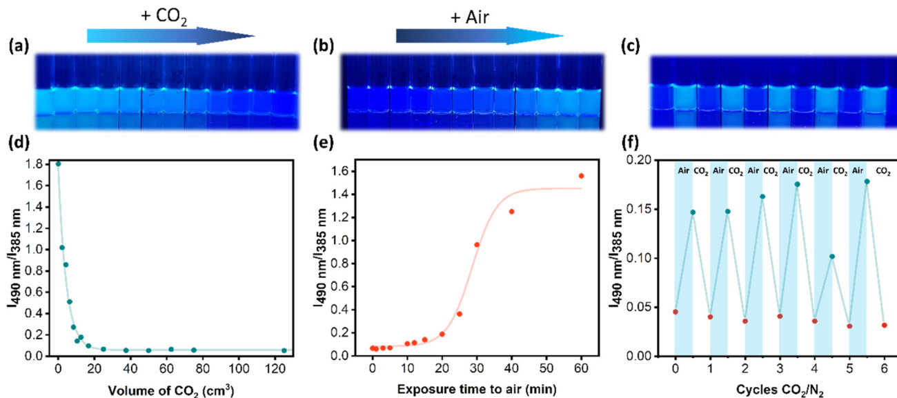
Fig. 3 (a) Photograph of P(DMAm-co-DEAPyMA) samples of concentration 0.01\text{ mg mL}^{-1} after bubbling different \text{CO}_2 volumes (OFF process) under 365\text{ nm} UV light. (b) Photograph of P(DMAm-co-DEAPyMA) samples of concentration 0.01\text{ mg mL}^{-1} after being exposed to atmospheric air for 1\text{ h} (ON process) under 365\text{ nm} UV light. (c) Photograph of P(DMAm-co-DEAPyMA) samples of concentration 0.01\text{ mg mL}^{-1} after undergoing several \text{CO}_2 /air cycles under 365\text{ nm} UV light. (d) Kinetics graphic representing a change in fluorescence intensity ratio I_{490\text{nm}}/I_{385\text{nm}} of a sample of concentration 0.01\text{ mg mL}^{-1} relative to the volume of \text{CO}_2 . (e) Kinetics graphic representing a change in fluorescence intensity ratio I_{490\text{nm}}/I_{385\text{nm}} of a sample of 0.01\text{ mg mL}^{-1} concentration when exposed to air for 1\text{ h} . (f) Graphic representing the change in fluorescence intensity ratio I_{490\text{nm}}/I_{385\text{nm}} of a sample of concentration 0.01\text{ mg mL}^{-1} when being exposed to \text{CO}_2 for 5\text{ min} and air for 1\text{ h} for 6 cycles.
