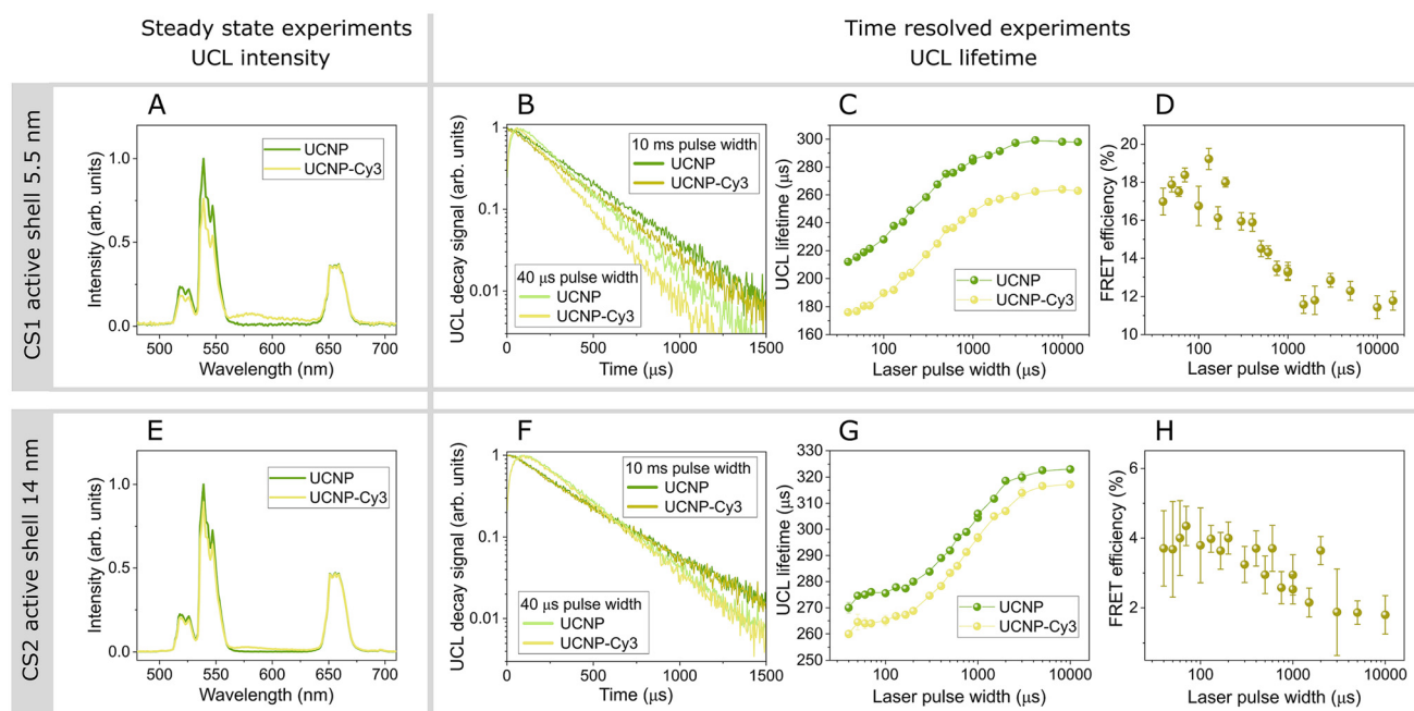
Fig. 2 (A) Green UCL emission spectra for a DMSO \text{NaYF}_4:\text{Yb},\text{Er} UCNP dispersion ( 0.5 \text{ mg mL}^{-1} ) (with and without Cy3) under 967 nm CW irradiation of 0.2 \text{ W} ( 444 \text{ W cm}^{-2} ). (B) Green (540 nm) UCL decay curves for two extreme representative excitation pulse widths ( 40 \mu\text{s} and 10 \text{ ms} ) in the case with and without Cy3, using an excitation laser power of 2.2 \text{ W} ( 5 \text{ kW cm}^{-2} ). (C) Green UCL lifetime as a function of the excitation pulse width for the sample with and without Cy3. Here, error bars are present but not discernible due to being smaller than the data point symbols. (D) FRET efficiency calculated from data of figure (C). (E)–(H) same as (A)–(D) for the UCNP with 14 nm active shell thickness.
