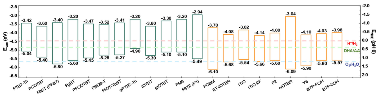
Fig. 22 Energy level alignment of conjugated polymers and small molecules for photocatalysts with redox potential of \text{H}^+/\text{H}_2 , DHA/AA, and \text{O}_2/\text{H}_2\text{O} .
