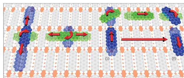
Fig. 15 Illustration of C_{22}H_{14} diffusion on C_{22}H_{14} /Cu(110) illustrating single ad molecules in potential energy minimum positions and the corresponding elementary diffusion processes. C_{22}H_{14} molecules preferentially move along the direction of their long axis (straight arrows, blue along \overline{\Gamma X} , green along \overline{\Gamma Y} ), but sometimes turn 90^\circ (curved arrows). The right-hand side shows a molecule that initially (position (i)) diffuses along \overline{\Gamma X} until it turns 90^\circ , moves along \overline{\Gamma Y} and finally (position (f)) turns back. The latter appears as a long jump along the \overline{\Gamma X} azimuth (long red arrow), covering multiple lattice distances, while it involves six individual steps. (Reprinted with permission from ref. 10 Copyright 2016 by Springer Nature).
