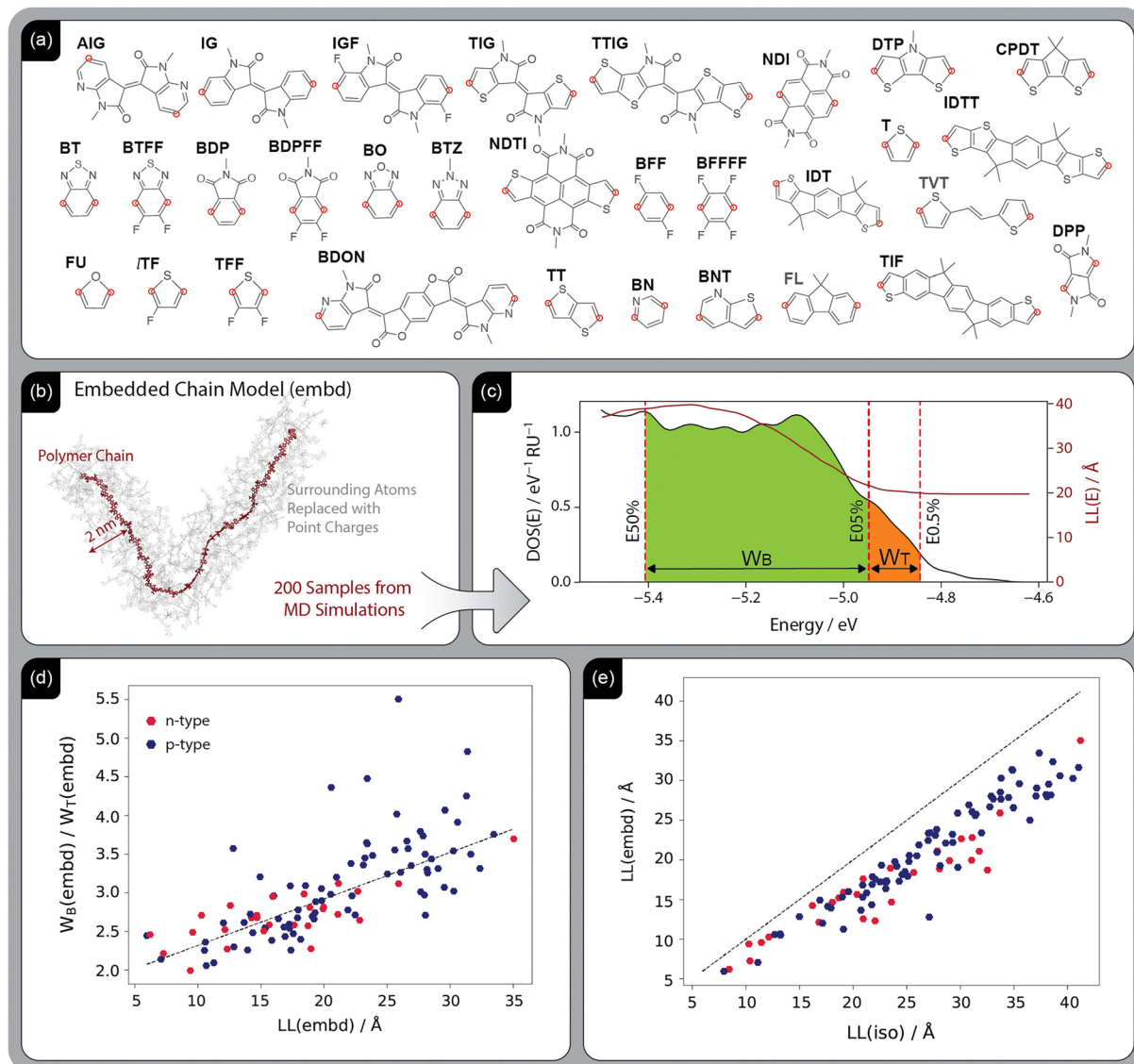
Fig. 1 (a) Structures and acronyms of monomers used in this study. CH 3 groups are used to indicate the connection with the alkyl side chain. (b) Schematic representation of the Embedded Chain (“emdb”) model used for DOS and LL calculations, as described in ref. 32. (c) Example results for a p-type polymer based on the Embedded Chain model, showing DOS(E) and LL(E) with definitions of key metrics: band-edge (E0.05%), tail-width ( W_T = |E_{0.5\%} - E_{0.05\%}| , highlighted in orange), and bandwidth ( W_B = |E_{50\%} - E_{0.5\%}| , highlighted in green). (d) Correlation graph between W_B/W_T and LL (Spearman’s rank correlation coefficient, S = 0.8 ). (e) Comparison of LL values calculated from the “emdb” and “iso” input models.
