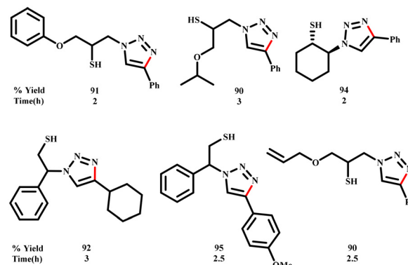
Scheme 5 \text{MgFe}_2\text{O}_4/\text{Cu} catalysed synthesis of \beta -thiol-1,4-disubstituted-1,2,3-triazoles from thiiranes (Eisavi et al. ).
