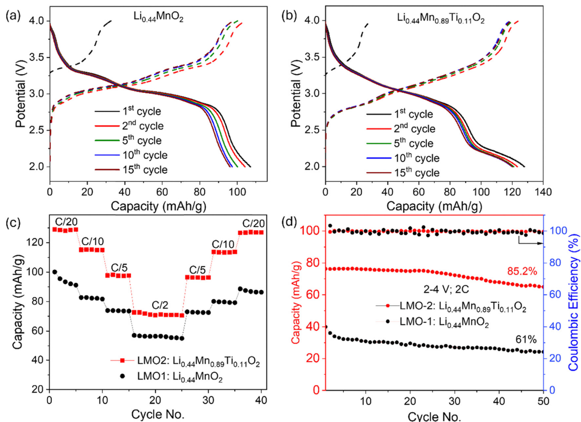
Fig. 4 Galvanostatic charge/discharge profiles for (a) pristine Li 0.44 MnO 2 (LMO1) and (b) Ti-doped Li 0.44 Mn 0.89 Ti 0.11 O 2 (LMO2) compositions cycled at a rate of C/20 (2–4 V). (c) Corresponding rate kinetics for LMO1 and LMO2. (d) Cycling stability and coulombic efficiency of LMO1 and LMO2 cycled at a fast rate of 2C in the voltage window of 2–4 V.
