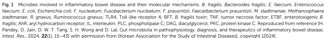
Fig. 1 summarizes the gut microbiota associated with the development and progression of IBD, as well as the related molecular mechanisms. 41 Due to the decreased abundance of the intestinal symbiotic flora, the loss of competition and antagonism against pathogenic bacteria provides an opportunity for the colonization of pathogens, leading to an overall shift in the gut microbiota characterized by a reduction in beneficial bacteria and an increase in harmful bacteria. 42 Fusobacterium mainly resides in the oral cavity and intestine. Compared with the healthy control group, the abundance of Fusobacterium in the colonic mucosa of UC patients is higher. Fusobacterium varium can cause colonic mucosal inflammation, exacerbating IBD. 43 Furthermore, due to the disruption of redox homeostasis in an inflammatory state, there is a surge in ROS/RNS levels. ROS/RNS provides terminal electron acceptors for anaerobic respiration, leading to a significant proliferation of facultative anaerobes and a decrease in the abundance of obligate anaerobes. 44 E. coli is a Gram-negative, facultative anaerobic bacterium. Evidence shows that the abundance of Adherent-invasive E. coli (AIEC) strains increases in the inflammatory state, and AIEC can adhere to and penetrate the intestinal mucosa of patients with IBD, thereby inducing inflammation and increasing the permeability of intestinal epithelium. 45 The decrease in the abundance of beneficial bacteria and the increase in harmful bacteria within the gut microbiota can lead to metabolic disorders, which are manifested primarily by the reduction of beneficial metabolites and the elevation of harmful metabolites. 46,47 The overall level of SCFAs in the intestines of patients with IBD is significantly reduced, mainly attributed to the reduced number of bacteria
