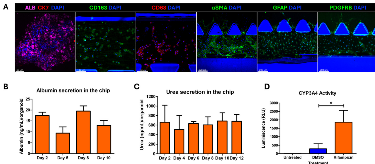
Fig. 4 Optimized growth conditions for co-culture of hepatobiliary organoids, iKCs and iHSCs on the LEADS chip. (A) Immunostaining of hepatobiliary organoids, iKCs and iHSCs on the LEADS chip in C1 medium after 10 days of co-culture on the chip. Markers indicating the differentiation and functional status of the different cell types were chosen for immunostaining. Albumin for hepatocytes; CK7 for biliary cells; CD163 and CD68 for iKCs; \alpha SMA, GFAP and PDGFRB for iHSCs. (B) Graph showing the amount of albumin secreted from the LEADS chip at the indicated days of co-culture quantified by ELISA. Error bars represent standard error of the mean. N = 3 experiments. (C) Graph showing the quantification of urea secretion from the LEADS chip at the indicated days of co-culture. Error bars represent standard deviation. N = 3 experiments. (D) Graph indicating the assessment of CYP3A4 enzyme activity. Error bars represent standard deviation. Paired t -test was performed. Rifampicin (induced) was compared against DMSO treatment (vehicle control). *p < 0.05 .
