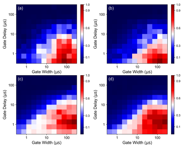
Fig. 4 SNR dependence on ICCD gate width and gate delay for (a) SP measurements of the Xe I 823.16 nm line, (b) DP measurements of the Xe I 823.16 nm line, (c) SP measurements of the Xe II 441.84 nm line, and (d) DP measurements of the Xe II 441.84 nm line.
