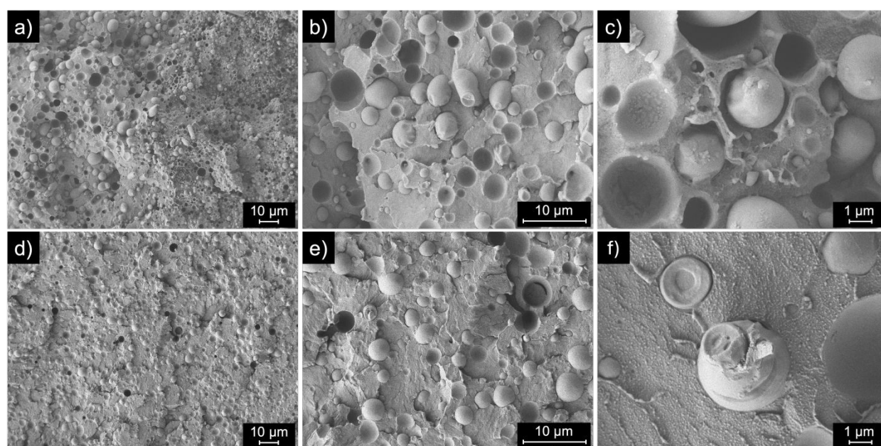
Figure 6. SEM images of fractured (a-c) control polymer blend and (d-f) 5 wt% plasma-oxidized LDPE polymer blend. The polymer blend is 70% LDPE (76 kg/mol) and 30% PLA with the addition of 5 wt% neat LDPE (40 kg/mol) acting as the control or plasma-oxidized LDPE (3.5%, oxygen incorporation, 40 kg/mol) acting as a compatibilizer. Plasma operating conditions for plasma-oxidized LDPE: treatment time: 2 h, O 2 feed molar percent: 2%, stir rate: 0 rpm, temperature: 150 °C, and LDPE to C 28 ratio of 1:1.
