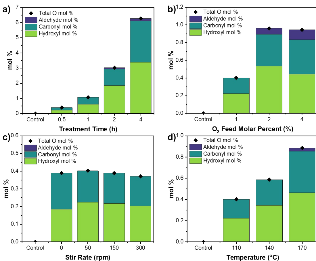
Figure 2. Oxygen percentages and type of functional group incorporation for neat and plasma-oxidized PEW at varying (a) treatment times, (b) O 2 feed molar percents, (c) stirring rates, and (d) temperatures. Carbonyl groups refer to middle chain C=O bonds while aldehyde groups refer to end chain C=O groups. Quantification from 1 H-
