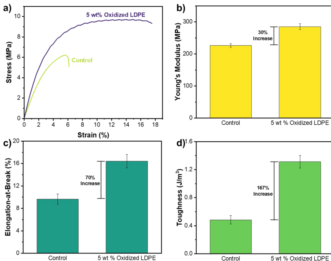
Figure 7. (a) Example stress-strain curve, (b) Young's Modulus, (c) elongation-at-break, and (d) toughness from tensile tests (10 %/min) of control and plasma-oxidized blends at 5 wt%. The polymer blend is 70% LDPE (76 kg/mol) and 30% PLA with the addition of 5 wt% neat LDPE (40 kg/mol) acting as the control or plasma-oxidized LDPE (3.5% oxygen incorporation, 40 kg/mol) acting as compatibilizer. Plasma operating conditions for plasma-oxidized LDPE: treatment time: 2 h, O 2 feed molar percent: 2%, stir rate: 0 rpm, temperature: 150 °C, and LDPE to C 28 ratio of 1:1. Errors represent the standard error across 6 replicates per sample type (n=6).
