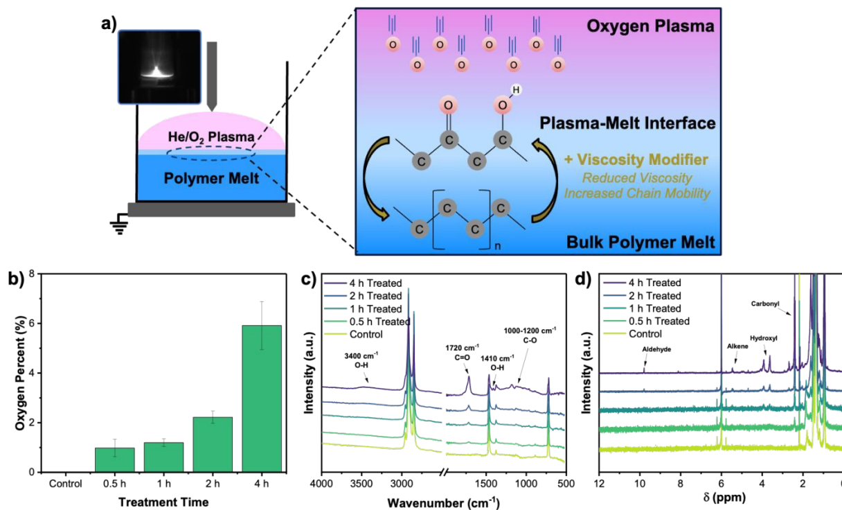
Figure 1. (a) Schematic of the plasma-melt interface in the pin-to-plate reactor with iCCD image of pulsed discharge. (b) XPS atomic percentages, (c) FTIR spectra, and (d) 1 H-NMR spectra of neat and plasma-treated PEW at various treatment times. Plasma operating conditions: O 2 feed molar percent: 1%, stir rate: 0 rpm, and temperature: 110 °C. XPS conditions: survey scan at 20 eV and 100 ms dwell time. FTIR conditions: MCTB detector at 4.0 cm -1 resolution and 32 scans. 1 H-NMR conditions: 115 °C in 1,1,2,2-tetrachloroethane-d 2 .
