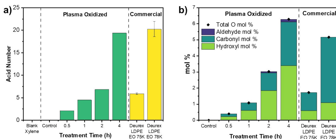
Figure 4. (a) Acid number and (b) corresponding oxygen percentages and functional group incorporation of neat, plasma-treated, and commercially oxidized waxes. Carbonyl groups refer to middle chain C=O bonds while aldehyde groups refer to end chain C=O groups. Plasma operating conditions: O_2 feed molar percent: 1%, stir rate: 0 rpm, and temperature: 110 °C.
