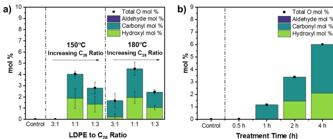
Figure 5. Oxygen percentage and functional group incorporation in plasma-treated LDPE (40 kg/mol) at various (a) LDPE to C 28 ratios at two temperatures and (b) treatment times at 150 °C and LDPE to C 28 ratio of 1:1. The control (neat LDPE) is also shown. Carbonyl groups refer to middle chain C=O bonds while aldehyde groups refer to end chain C=O groups. Plasma operating conditions: treatment time: 2 h, O 2 feed molar percent: 2%, stir rate: 0 rpm.
