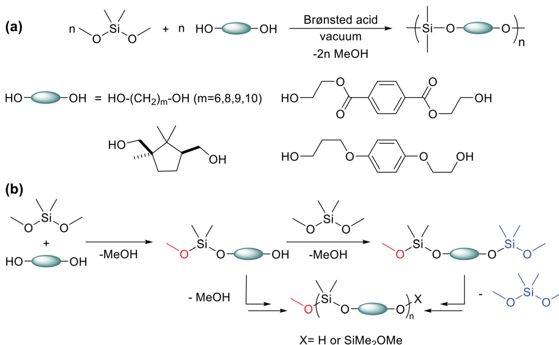
Fig. 4 Polycondensation of dimethoxydimethylsilane with different diols (a), and the plausible mechanism (b). 20
