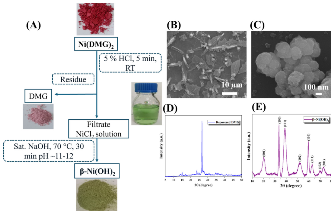
Fig. 6 (A) The flowchart for the recovery of Ni and DMG from the spent \text{LiB} -derived \text{Ni}(\text{DMG})_2 complex. (B and C) FE-SEM morphology of recovered DMG and \beta\text{-Ni}(\text{OH})_2 . (D and E) Powder XRD of recovered DMG and \beta\text{-Ni}(\text{OH})_2 .
