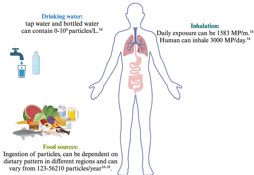
Fig. 1 Exposure to MNPs through the common routes. According to the WHO and EFSA report, human can be exposed to different amounts of MNPs in their daily life through various routes, particularly by ingestion and inhalation. 16-18
