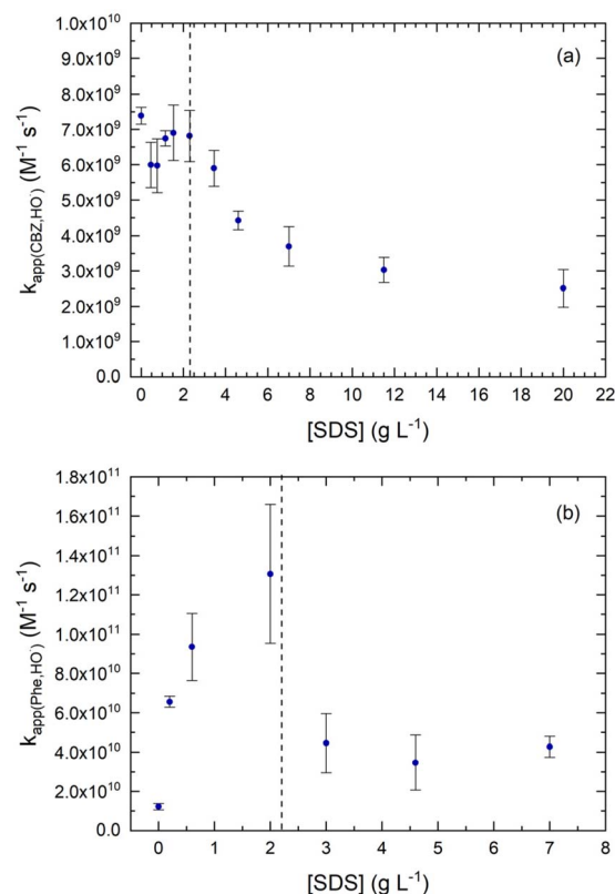
Fig. 2 Apparent second-order rate constant for the reaction of hydroxyl radicals with (a) CBZ and (b) Phe as a function of SDS concentration. Error bars correspond to the uncertainty estimated based on the standard deviation of replicate measurements and the uncertainty associated with the k_{\text{TPA},\text{HO}\cdot} value. The vertical dashed line indicates the CMC of SDS.
