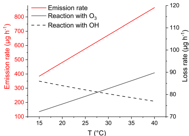
Fig. 5 Temperature-dependent limonene emission rate from wooden furniture (81 m 2 ) in the test house (room volume 46 m 3 ), and loss rate due to reaction with ozone (6 μg m -3 ) and OH radicals (1 × 10 5 molecules per cm) at a limonene concentration of 22 μg m -3 .
