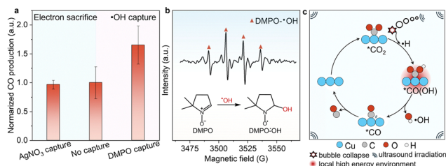
Fig. 5 Investigation on the mechanism of sonocatalytic \text{CO}_2 -to-CO conversion using \text{r-Cu}_{0.8}/\text{ZnAl-LDO} . (a) The comparison of CO production in the presence of radical or electron trap. (b) Measured electron paramagnetic resonance (EPR) spectrum of the solution with addition of DMPO after ultrasound irradiation. (c) Proposed mechanism for CO production.
