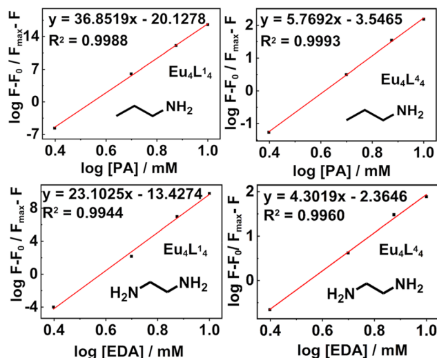
Fig. 5 Linear range of \log F - F_0/F_{\max} - F for \text{Eu}_4\text{L}_4 and \text{Eu}_4\text{L}_4 towards \log[\text{amine}] . The reciprocal of the intercept of the linear regressions is the binding constant of \text{Eu}_4\text{L}_4 and \text{Eu}_4\text{L}_4 .
