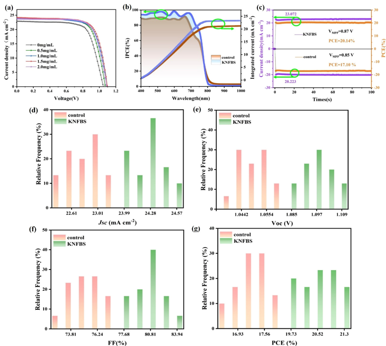
Fig. 2 Photovoltaic performance of pristine and KNFBS-treated devices: (a) J-V curves; (b) IPCE curves. (c) Stabilized PCE and J_{sc} at the maximum power point (MPP) output. Statistical photovoltaic parameter distribution obtained from 30 devices: (d) J_{sc} ; (e) V_{oc} ; (f) FF; (g) PCE.
