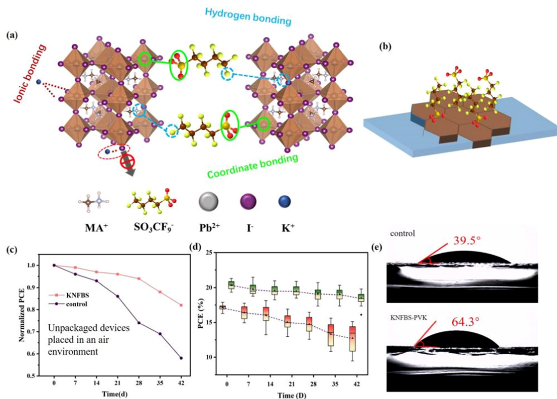
Fig. 6 Schematic of the KNFBS-treated perovskite with multifunctional passivation: (a) chemical interaction between KNFBS molecules and the perovskite, and (b) suppression of ion migration and trap mitigation at GBs. Long-term stability tests of the unencapsulated control and KNFBS-doped devices stored in open air conditions at room temperature with a RH of 35 \pm 5\% in the (c) champion devices and (d) corresponding statistical distribution extracted from 30 cells. (e) Water contact angles deposited on control and KNFBS-doped perovskite films.
