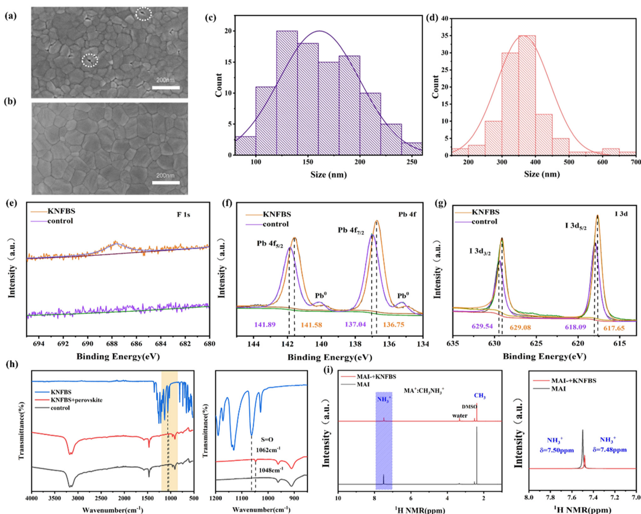
Fig. 3 Top-view SEM images of (a) pristine and (b) KNFBS + perovskite films. Histograms of the grain size of (c) pristine and (d) KNFBS + perovskite films. XPS spectra of control and KNFBS-doped perovskite films: (e) F 1s; (f) Pb 4f and (g) I 3d. (h) FTIR spectra of pure KNFBS passivators, pristine, KNFBS-doped perovskites. (i) NMR spectra of the MAI and mixed MAI + KNFBS in DMSO- d_6 solutions.
