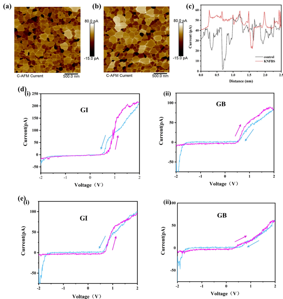
Fig. 4 c-AFM mapping of the currents at perovskite GBs and grains. Current images for (a) the control, (b) KNFBS-doped perovskite films, and (c) current distribution based on random 1D line scanning. Distinct I - V hysteresis at the GI or GBs for (d) the control and (e) KNFBS-doped perovskite films, respectively.
