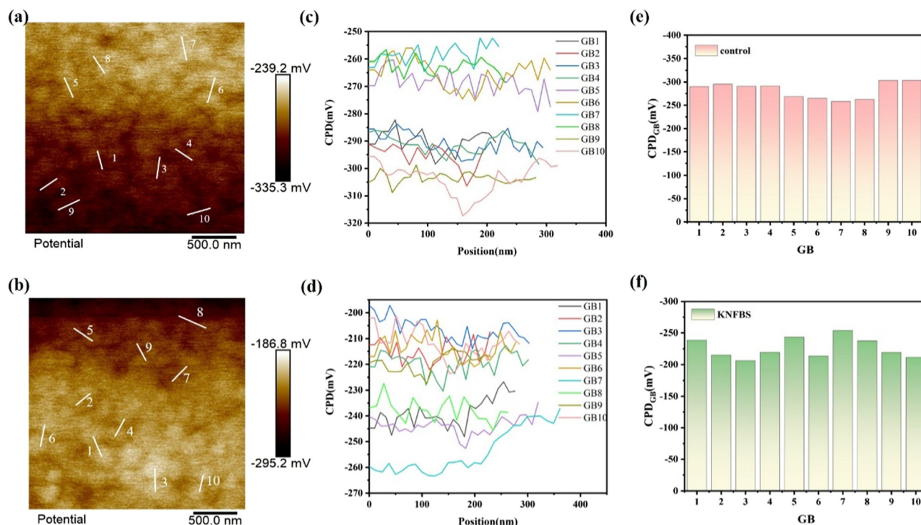
Fig. 5 (a) and (b) Contact potential difference (CPD) image of KPFM mapping. The recorded lines mark the different measured location of GBs. (c) and (d) The profiles based on 1D line scanning of the previous CPD image. (e) and (f) Statistical CPD variation across the GBs based on the corresponding 1D line scanning profiles. The diagrams in the first and second lines are for the control and KNFBS-doped perovskite films, respectively.
