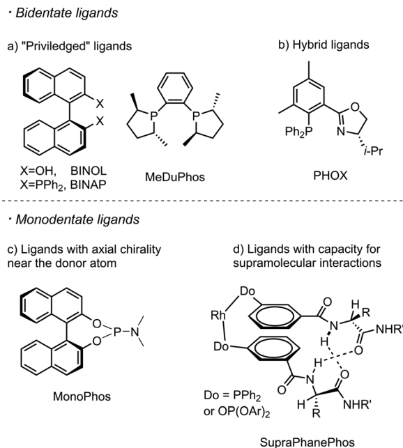
Fig. 1 Types of ligands applied in enantioselective hydrogenation. Bidentate: (a) "privileged" ligands, (b) hybrid ligands. Monodentate: (c) ligands with axial chirality near the donor atom, (d) ligands with capacity for supramolecular interactions.
