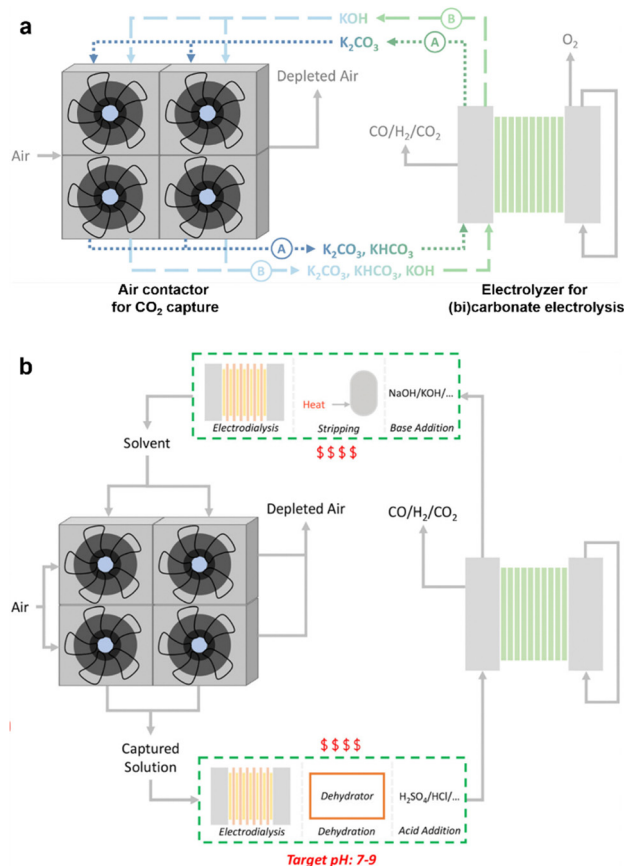
Fig. 13 Schematic of the integration route proposed in the literature, with the air contactors on the left and the electrolyzer stacks on the right. (a) The two pathways for CO 2 capture from the air are (A) K 2 CO 3 -based and (B) KOH-based. (b) Potential solutions to address the different pH requirements of the capture and conversion processes are shown inside the green dashed boxes at the top and bottom. Reproduced with permission from ref. 168.
