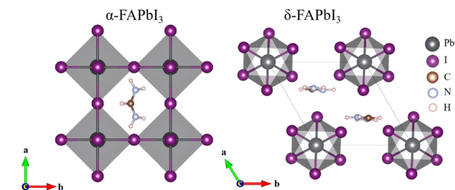
Fig. 1 Structures of FAPbI 3 for different phases.
