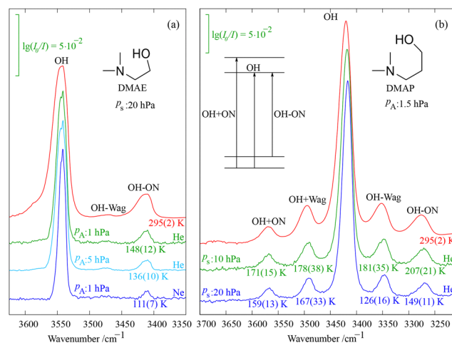
Fig. 6 Estimated vibrational temperature T_v in K of low frequency hydrogen bond stretching (ON) and dimethylamino wagging (Wag) modes in soft supersonic jet expansions of partial pressure p_A as a function of carrier gas for DMAE (a) and as a function of stagnation pressure p_s for DMAP (b) derived from reference room temperature spectra (red). See text and ESI,† Section S3, in addition to Tables S10–S12 for further explanations.
