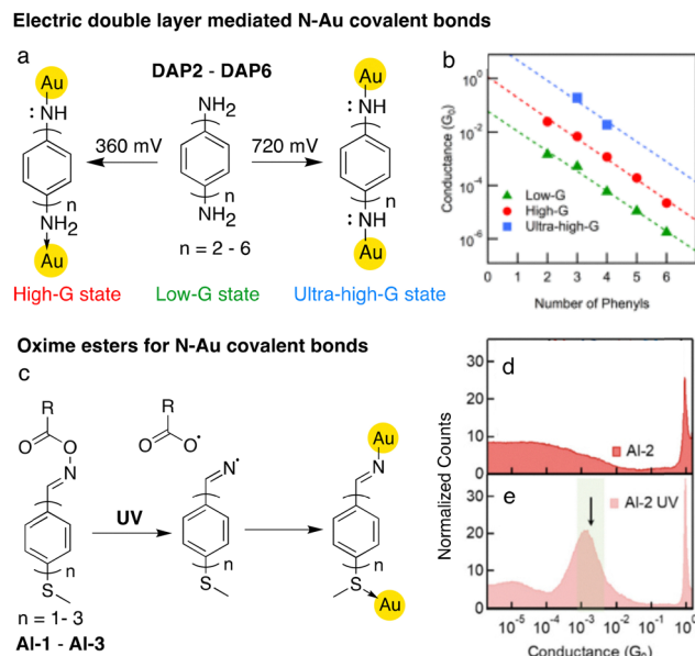
Fig. 4 (a) Schematic illustration of the formation of the novel N–Au contact upon oxidation of a dative N→Au bond under high bias voltage in an ionic environment with a wax-coated STM tip. (b) The most probable conductance values, determined from Gaussian fits to peaks in 1D conductance histograms, as a function of the number of phenylene units in the molecular backbone. Data were acquired at a constant tip bias of 90 mV for low-G, either 360 or 720 mV for high-G, and 720 mV for ultra-high-G. Dashed lines are linear fits to these data. (c) Illustration of the iminyl radical–Au covalently bonded single-molecule junctions. 1D conductance histograms of (d) Al-2 and (e) UV-light-treated Al-2 measured in propylene carbonate (PC) with a wax-coated STM tip under a tip bias voltage of 0.5 V. (b) is reprinted with permission from ref. 67, copyright (2017) American Chemical Society. (d) and (e) are adapted with permission from ref. 55, copyright (2023) American Chemical Society.
