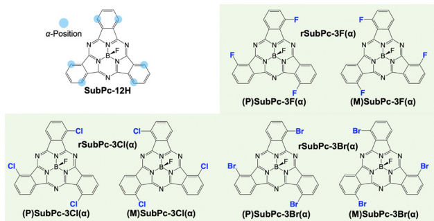
Fig. 1 Chemical structures of chiral subphthalocyanine (SubPc) derivatives with a schematic illustration of the \alpha -positions of SubPc.
