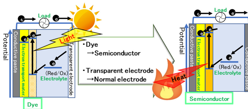
Fig. 2 Schematic image of a dye-sensitized solar cell and a semiconductor-sensitized thermal cell. Mater.: material.
