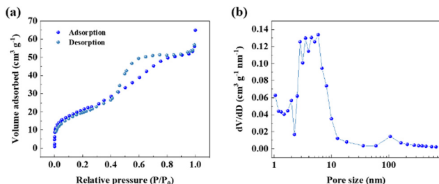
Fig. 3 (a) \text{N}_2 adsorption-desorption isotherm; and (b) BJH pore-size distribution of Sn@NC.
