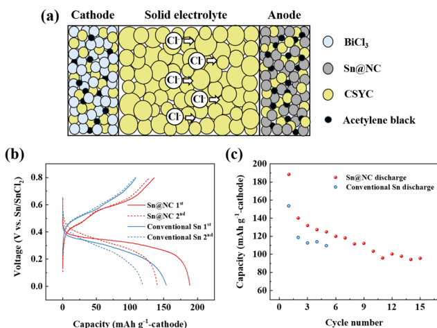
Fig. 4 (a) Schematic diagram of the all-solid-state \text{Cl}^- -ion battery; (b) charge-discharge profiles; and (c) cycling performance of the Sn@NC/CSYC/ \text{BiCl}_3 and conventional Sn/CSYC/ \text{BiCl}_3 cells.
