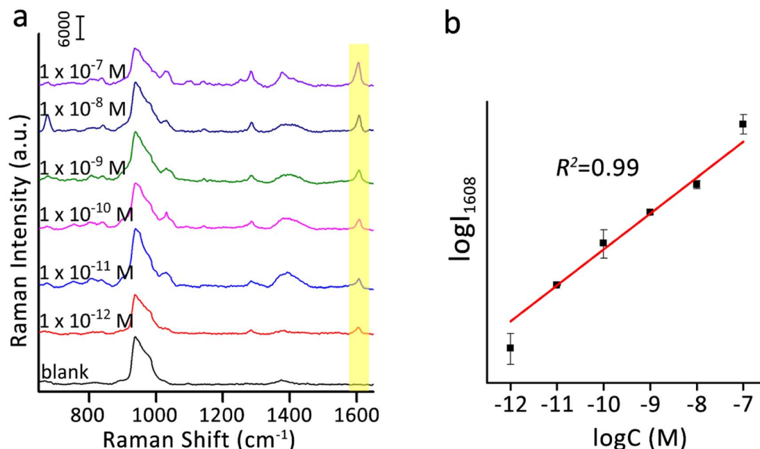
Fig. 6 (a) 10^{-7} to 10^{-12}\text{ M} concentrations of PCB-77 are detected on the C-NR@Ag substrate. (b) Correlation between the log–log plot of I_{1608} and C_{\text{PCB-77}} . The error bar was obtained by three replicate determinations.
