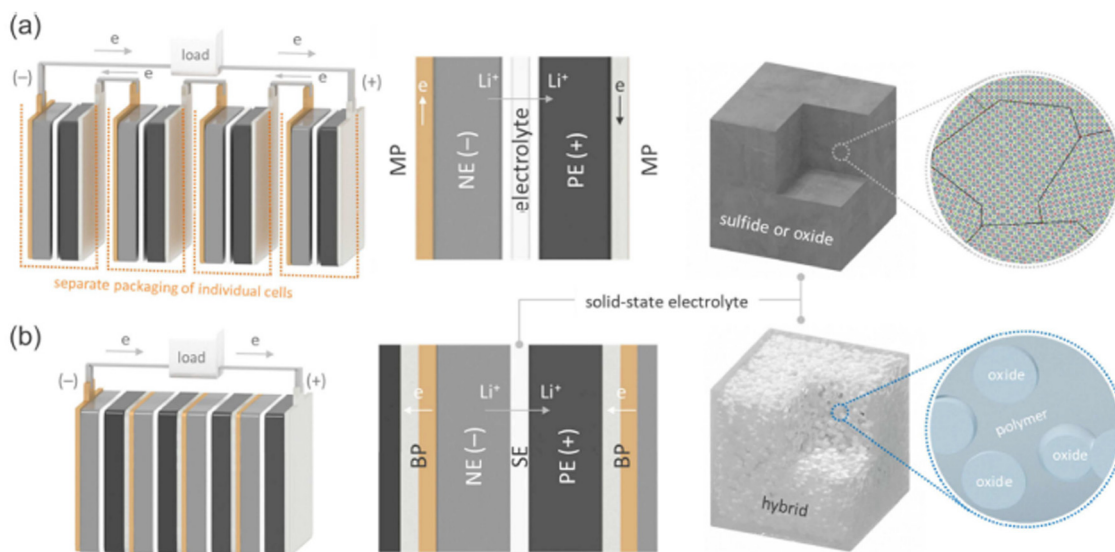
Fig. 10 Schematic diagrams of (a) the monopolar design of current LIBs with liquid electrolytes and (b) bipolar design of SSLBs equipped with SEs. The Li + and electron pathways during discharge are also indicated. (Reproduced with permission from ref. 63).
