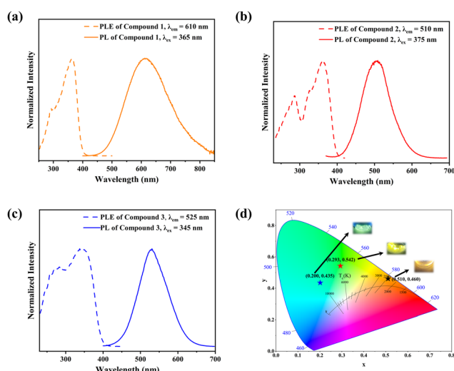
Fig. 2 (a), (b) and (c) PLE and PL spectra at room temperature. The solid lines are the emission spectra at different excitation wavelengths. The dashed lines are the excitation spectra at different emission wavelengths. (d) CIE chromaticity coordinates corresponding to 1 , 2 and 3 . Inset: Photographs of the compounds under UV light.
