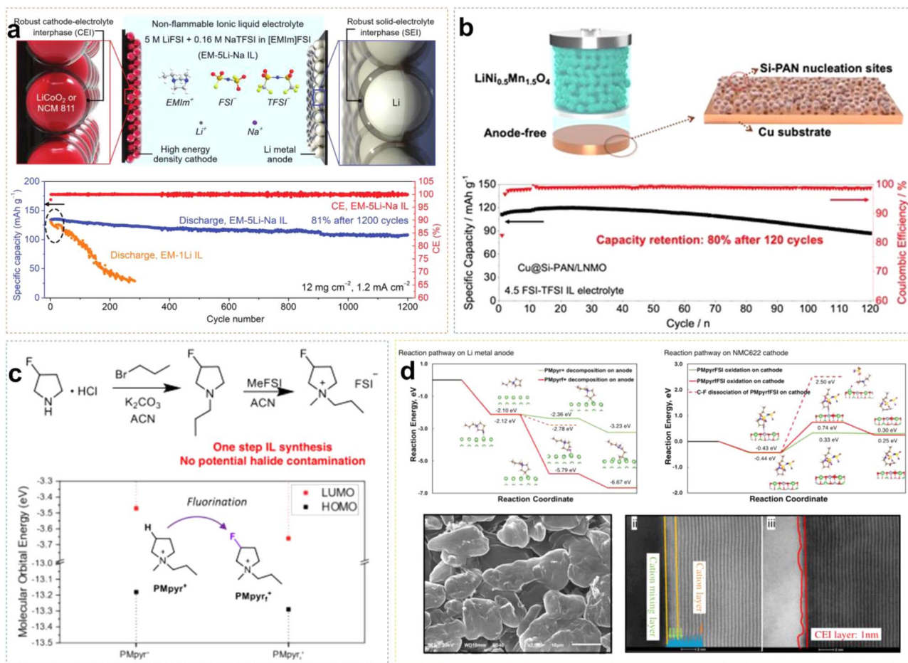
Fig. 4 (a) Schematic diagram of robust EEL formed by EM-5Li-Na ILE and corresponding cycling performance in Li/LCO cells with the mass loading of 12 mg cm -2 . Reprinted from ref. 37 with permission. Copyright 2020, Wiley. (b) Schematic illustrations of the high-voltage LNMO anode-free batteries using the Cu@Si-PAN current collector, and corresponding cycling performance of the LNMO anode-free batteries with 4.5 FSI-TFSI ILE. Reprinted from ref. 38 with permission. Copyright 2022, Wiley. (c) Synthesis route for PMpyr + FSI and comparison of HOMO/LUMO energy levels for PMpyr + and PMpyr + . (d) PMpyr + and PMpyr + reduction and oxidation pathway on Li metal and NMC622 cathode, respectively; the morphology of plated Li on Cu foil and HAADF-STEM analysis of cycled NMC622 cathodes. Reprinted from ref. 39 with permission. Copyright 2023, Springer Nature.
