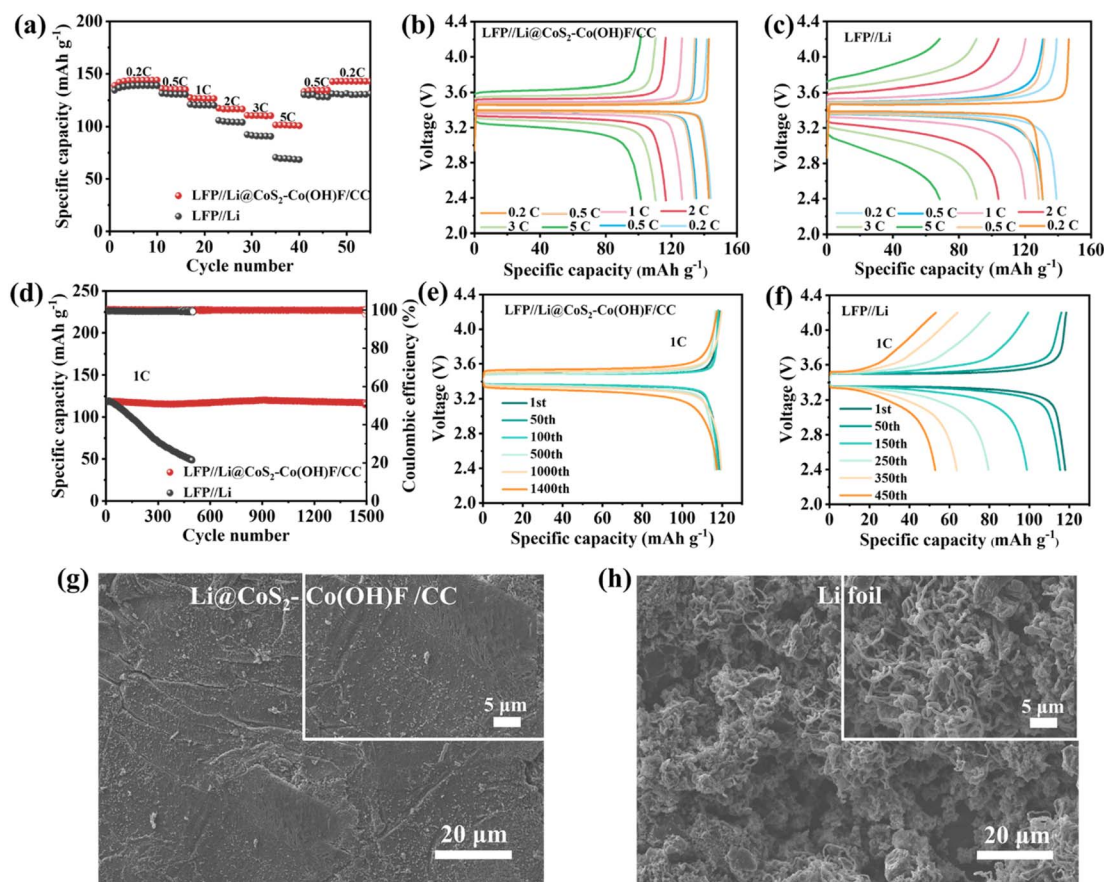
Fig. 7 (a) Rate capability and (b and c) charge–discharge profiles of LFP//Li@Li@CoS 2 –Co(OH)F/CC and LFP//Li full cells at various rates ranging from 0.2C to 5C. (d) Cycle performance and (e and f) charge–discharge profiles of LFP//Li@CoS 2 –Co(OH)F/CC and LFP//Li full cells at 1C. The SEM images of the corresponding anode for (g) LFP//Li@CoS 2 –Co(OH)F/CC and (h) LFP//Li full cells after 200 cycles at 1C.
