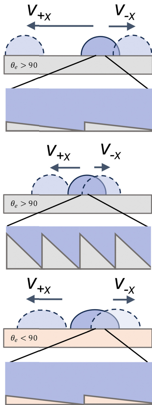
Fig. 6 (top) Low angled surfaces have anisotropic pinning with high velocities in the +x direction and low velocity in the -x direction. (middle) High angled surfaces show strong pinning in both directions with low droplet velocities in the +x and -x directions. (bottom) Hydrophilic surfaces with anisotropic pinning with lower contact angles and velocities.
