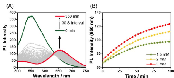
Fig. 5 (A) Time-dependent PL spectra of Pt-L 1 (2.0 mM, \lambda_{\text{ex}} = 420 nm) in the presence of Fe(BF 4 ) 2 (1.5 equiv.) in DMSO/H 2 O (9:1 v/v) at 293 K. (B) Plots for PL intensity at 650 nm vs. time at different concentrations of Pt-L 1 (1.5–3.0 mM) in the presence of Fe(BF 4 ) 2 (1.5 equiv.).
