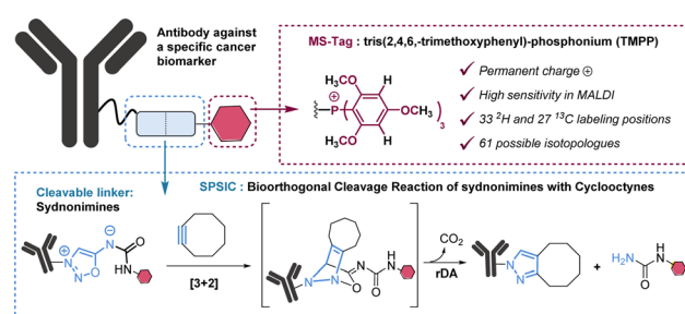
Fig. 2 Bioconjugates used in this study. Our strategy is based on the combination of two technologies: the multiplexed MS-detection of TMPP- isotopologues and sydnonimine cleavable linkers. rDA: retro-Diels-Alder.
